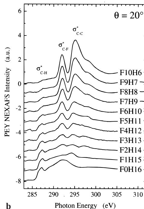
Figure 10. PEY NEXAFS spectra of SF-SAM (Au) samples at EGB = -150 V and (a) \theta = 90^\circ and (b) \theta = 20^\circ . In the nomenclature used, FyHx corresponds to a \text{HS}(\text{CH}_2)_{16-y}(\text{CF}_2)_y\text{F} moiety.
