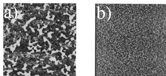
Figure 7. Scanning force microscopy images of the surfaces of BC-F8H4 cast from (a) \alpha,\alpha,\alpha -trifluorotoluene, and (b) a 50/50 (w/w) \alpha,\alpha,\alpha -trifluorotoluene/toluene mixture. The length of the edge of each picture corresponds to 30 \mu\text{m} .
